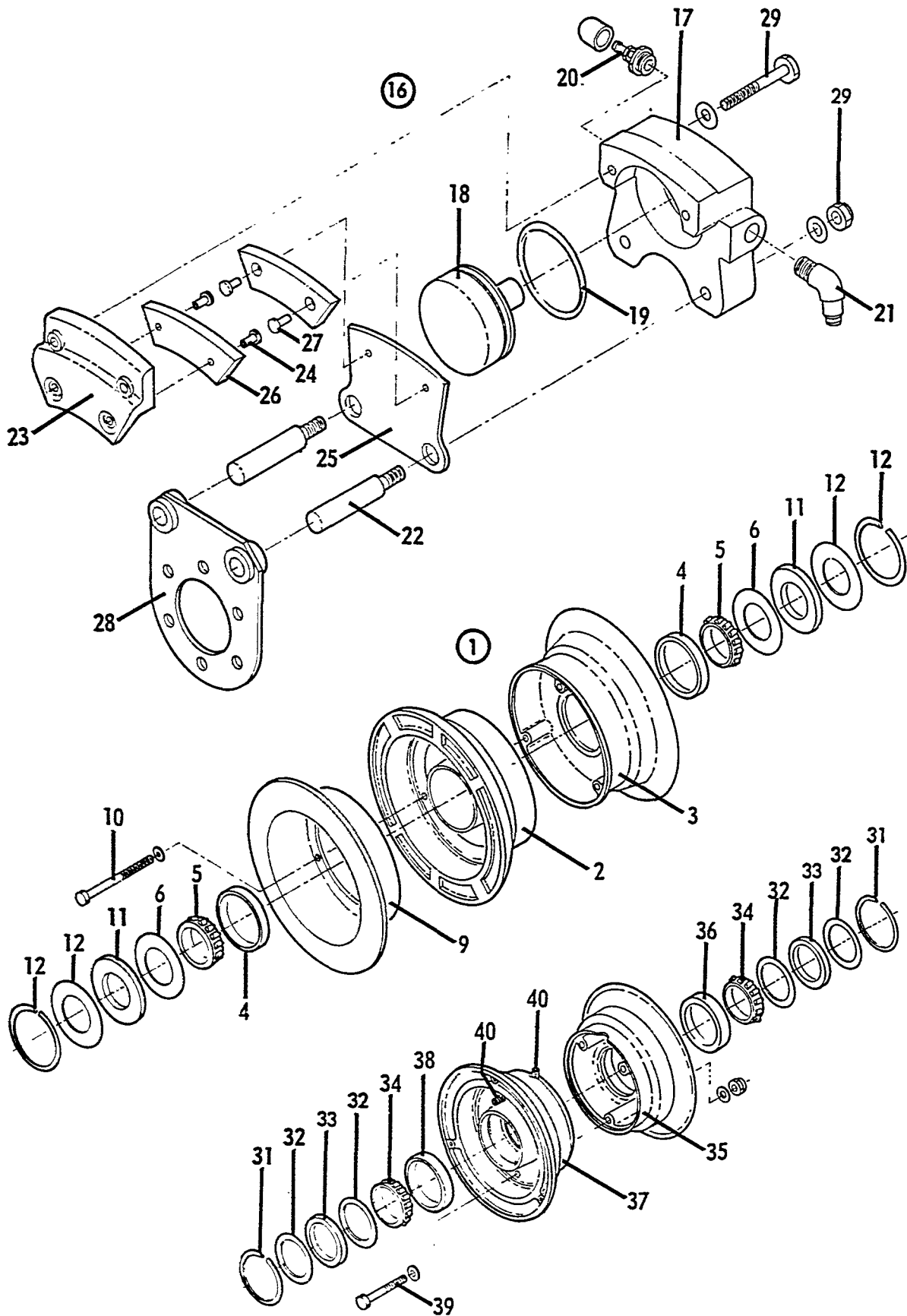
FIGURE 24. Wheel & Brake Assemblies
