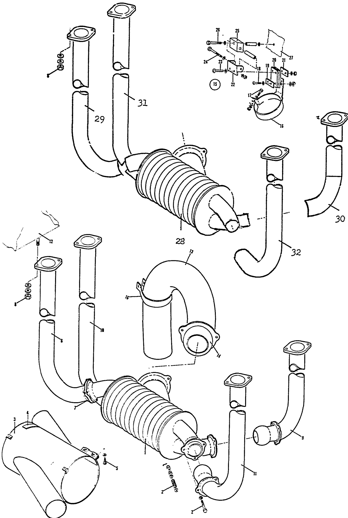
Figure 35A, Mooney Exhaust Systems
