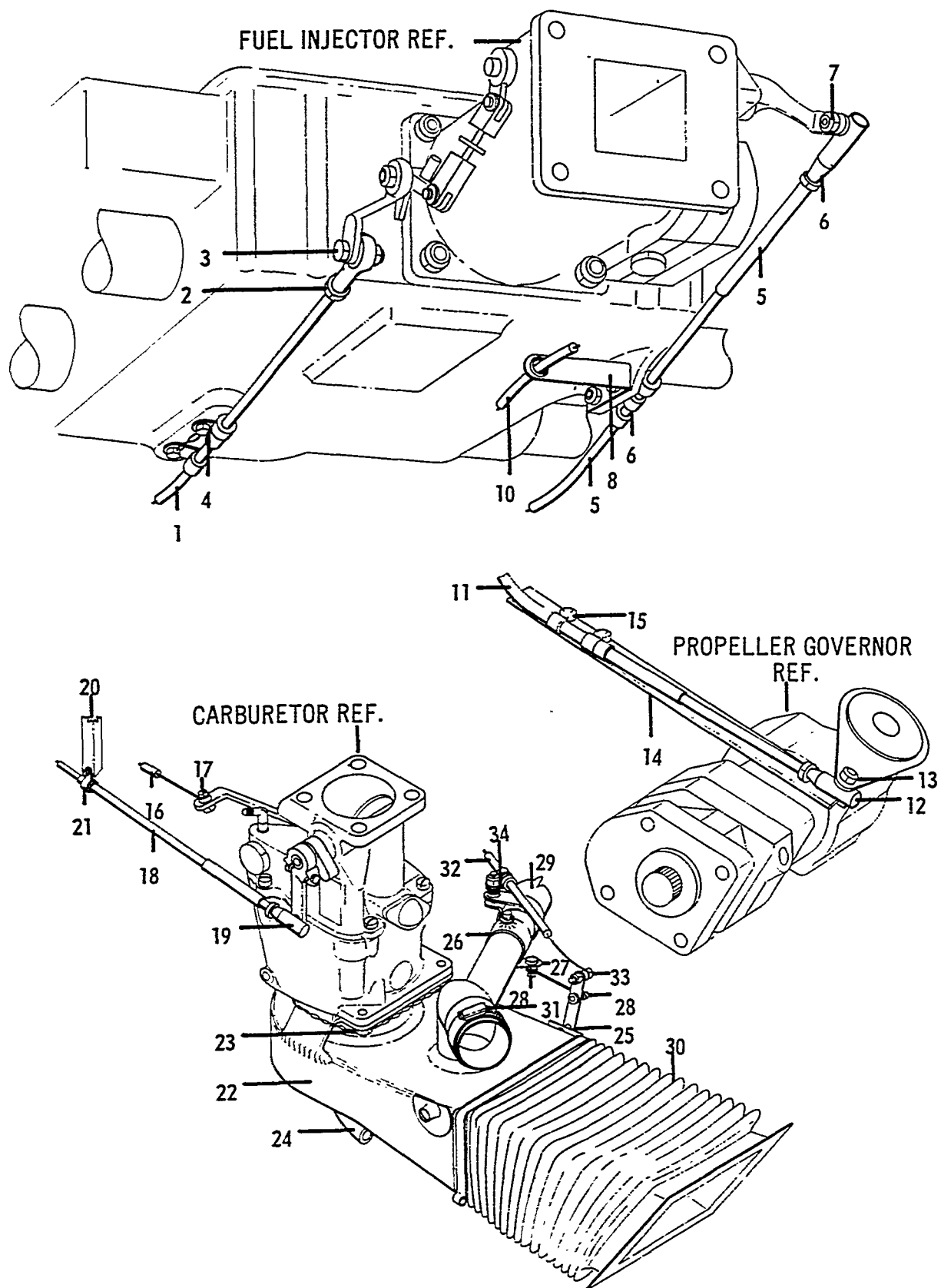
FIGURE 36. Engine Controls
