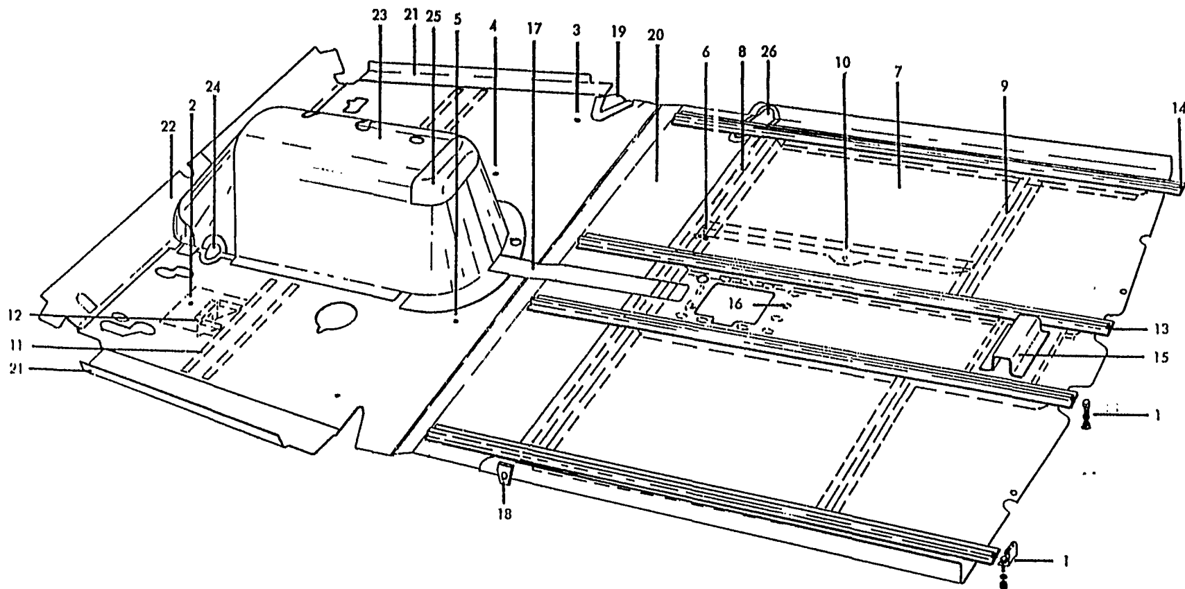
FIGURE 9. Fuselage Floorboard Assembly
