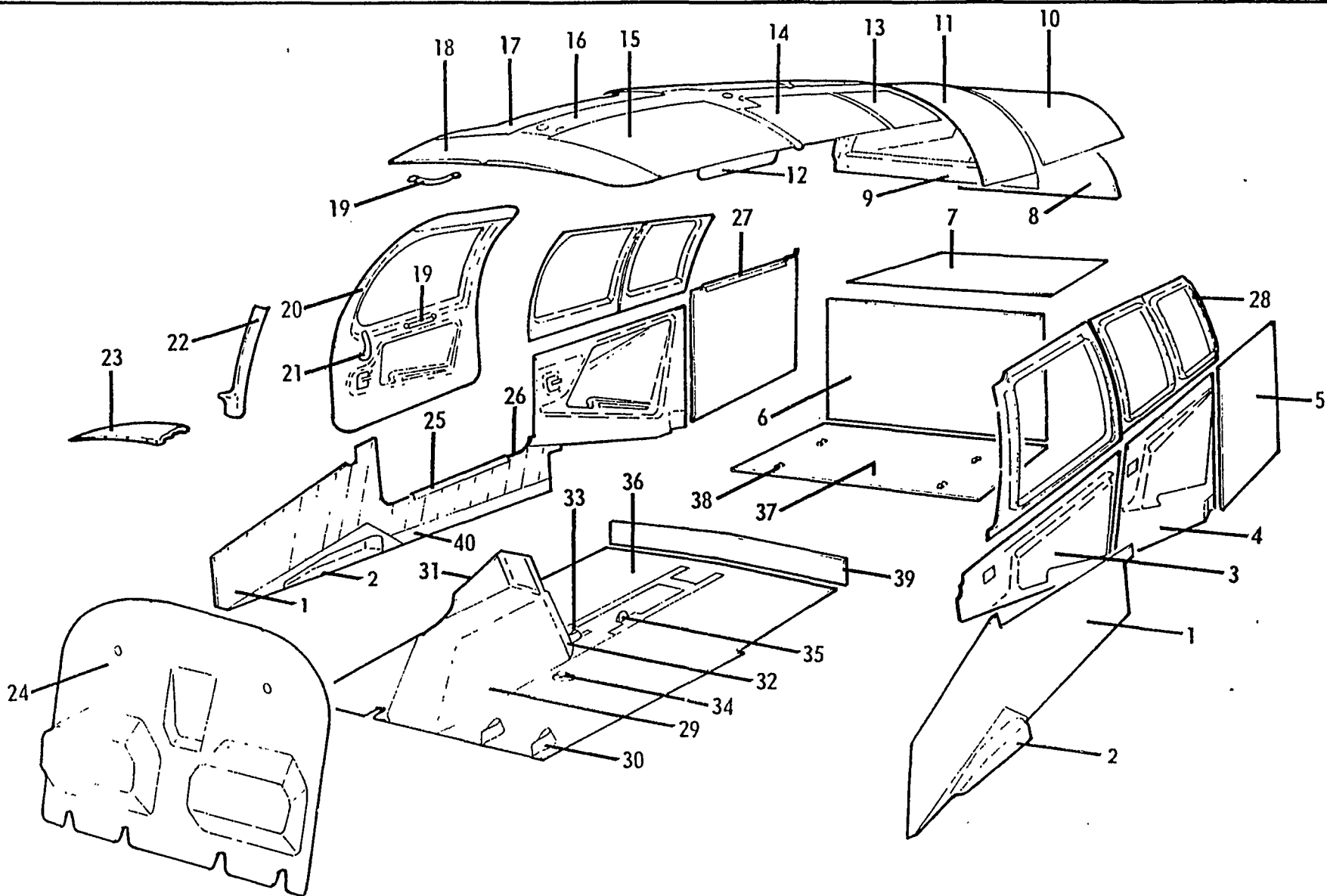
FIGURE 46. Cabin Interior Furnishings (M20F)
