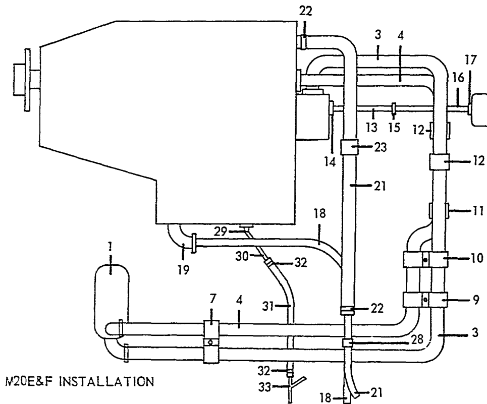
FIGURE 38. Engine Oil System
