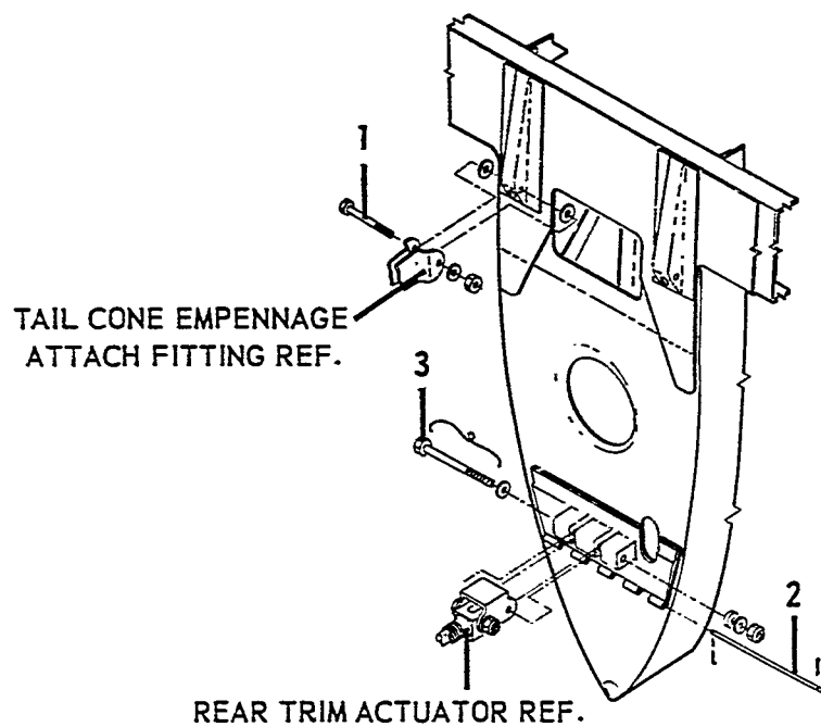
FIGURE 18. Empennage Assembly & Installation
