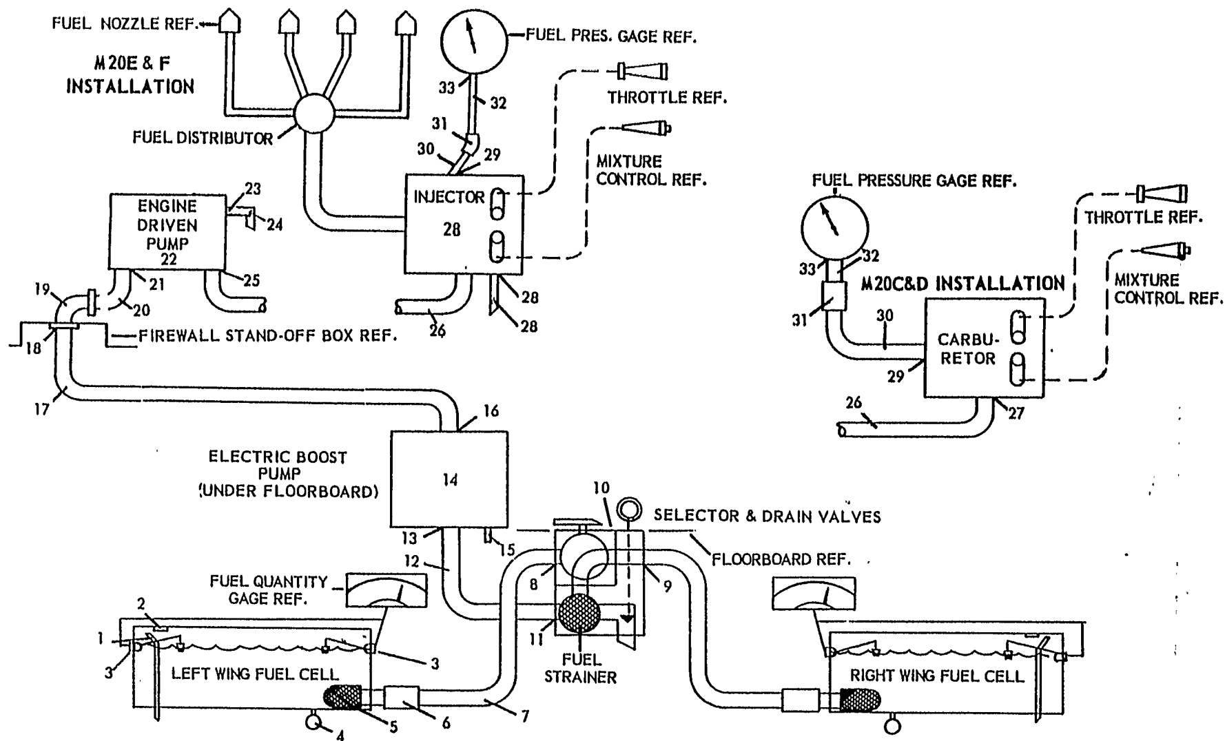
FIGURE 37. Engine Fuel System
