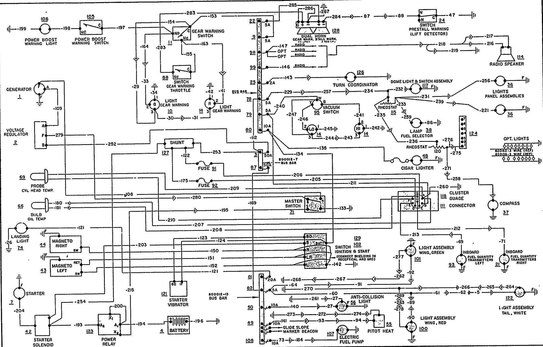
FIGURE 50H. Electrical System (1967 & ON M20E)
