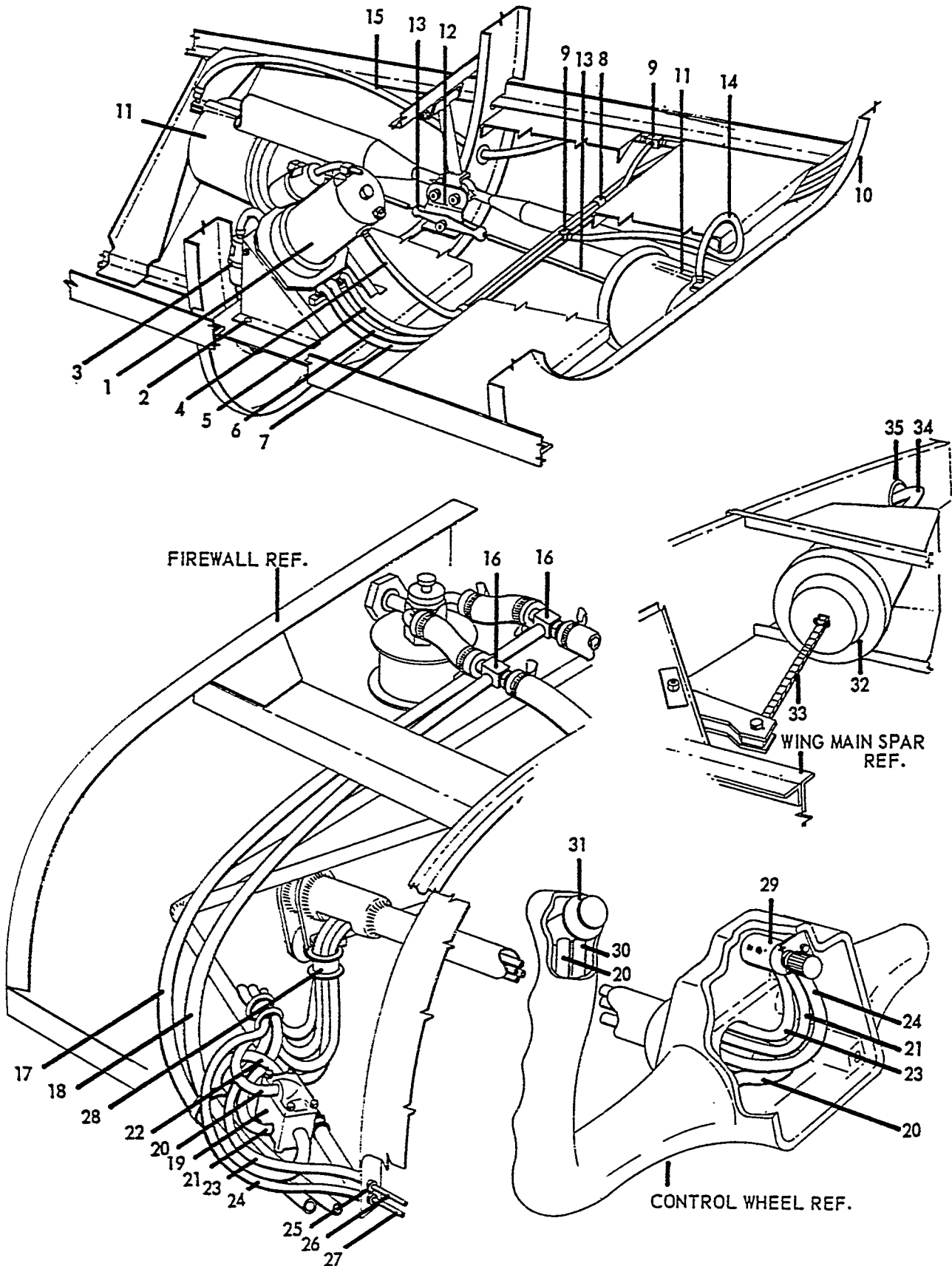
FIGURE 31. Positive Control System (1965)
