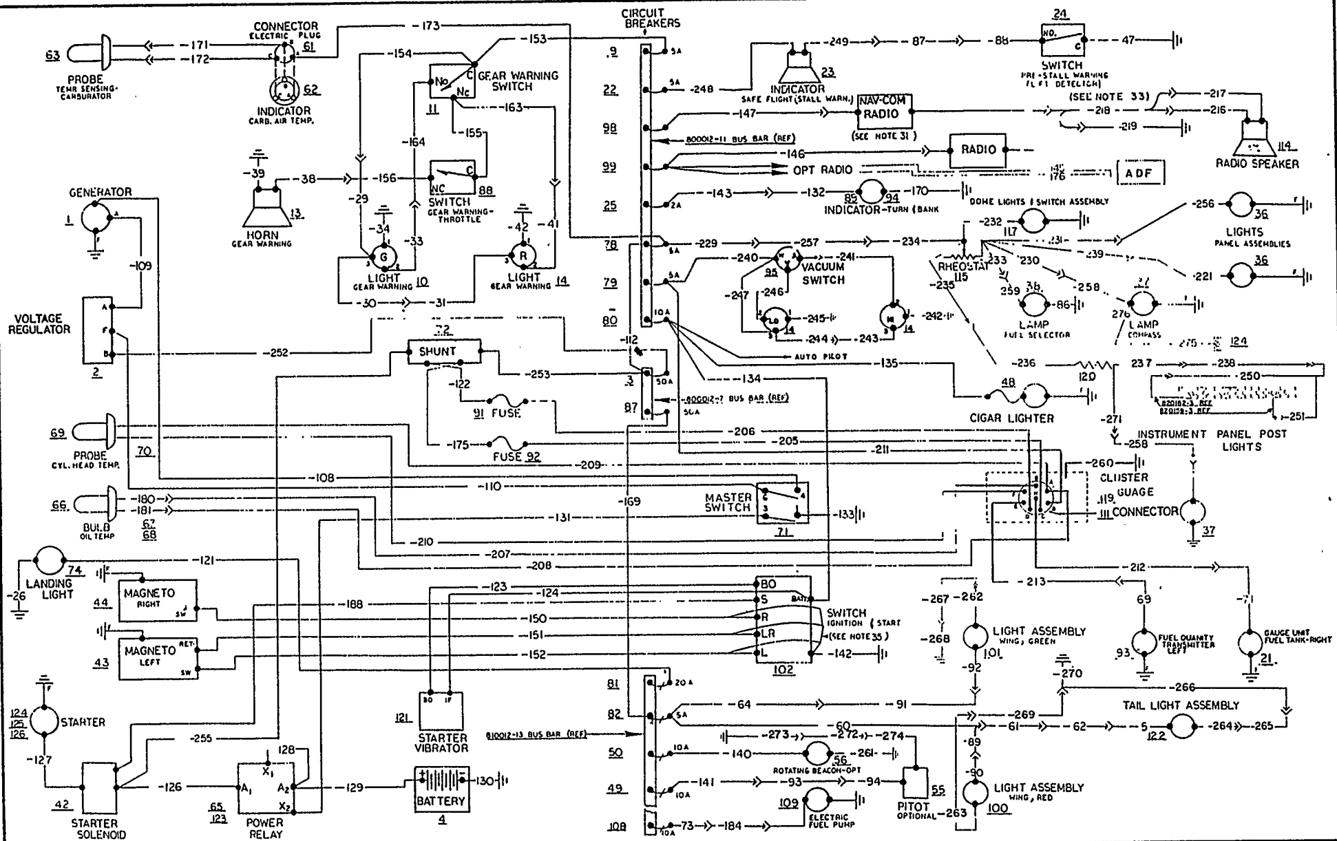
FIGURE 50D. Electrical System (1966 M20C)
