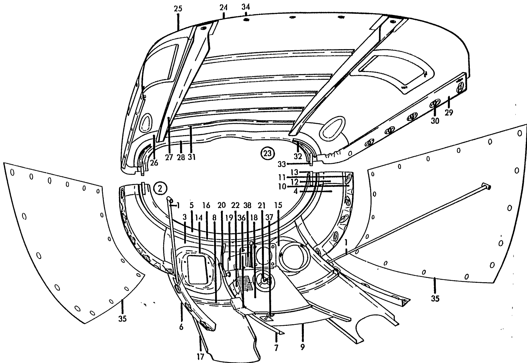
FIGURE 41. Engine Cowling Assembly (1965)
