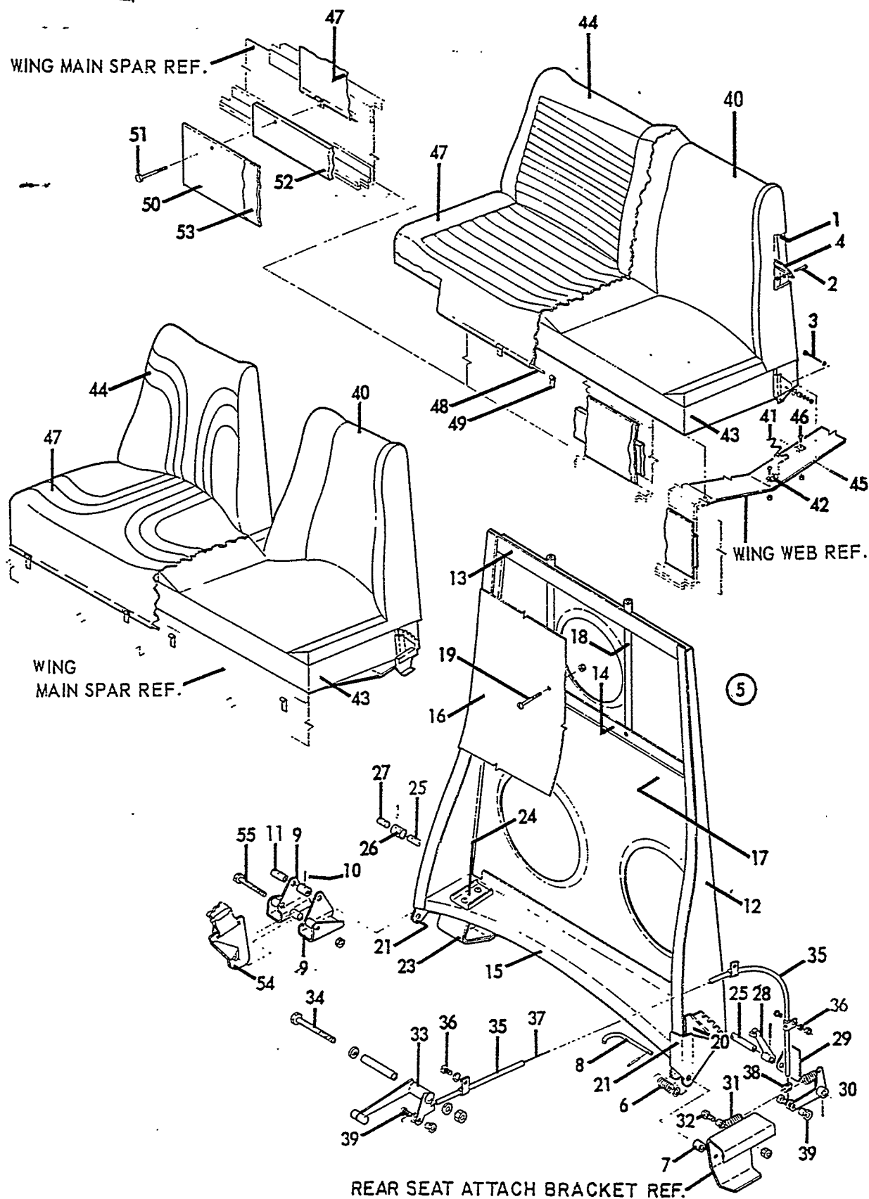
FIGURE 48. Rear Seat Assemblies
