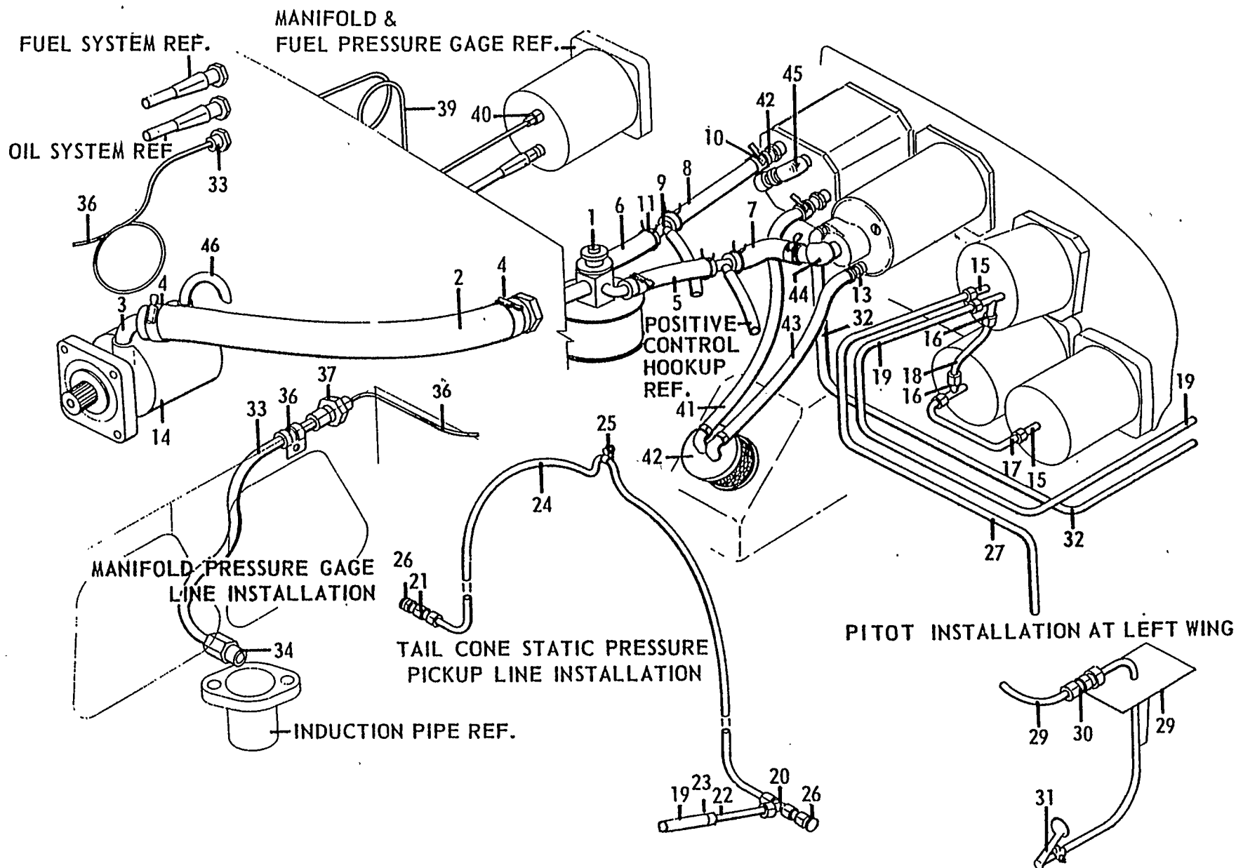
FIGURE 53. Vacuum, Manifold & Static Pressure Systems
