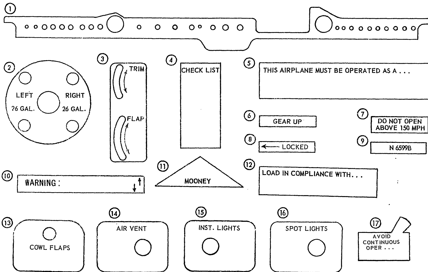
FIGURE 49 Interior Placards &amp; Decals
