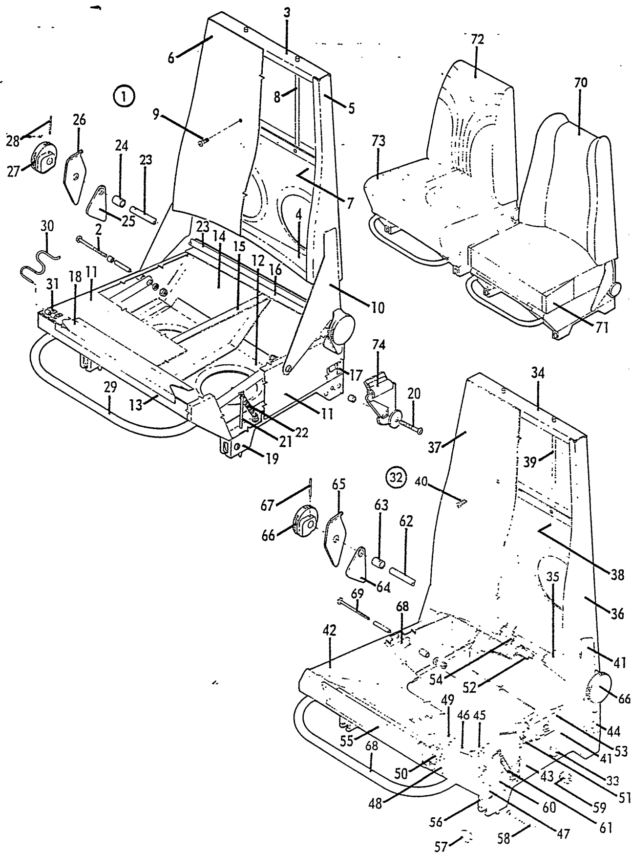
FIGURE 47. Front Seat Assemblies
