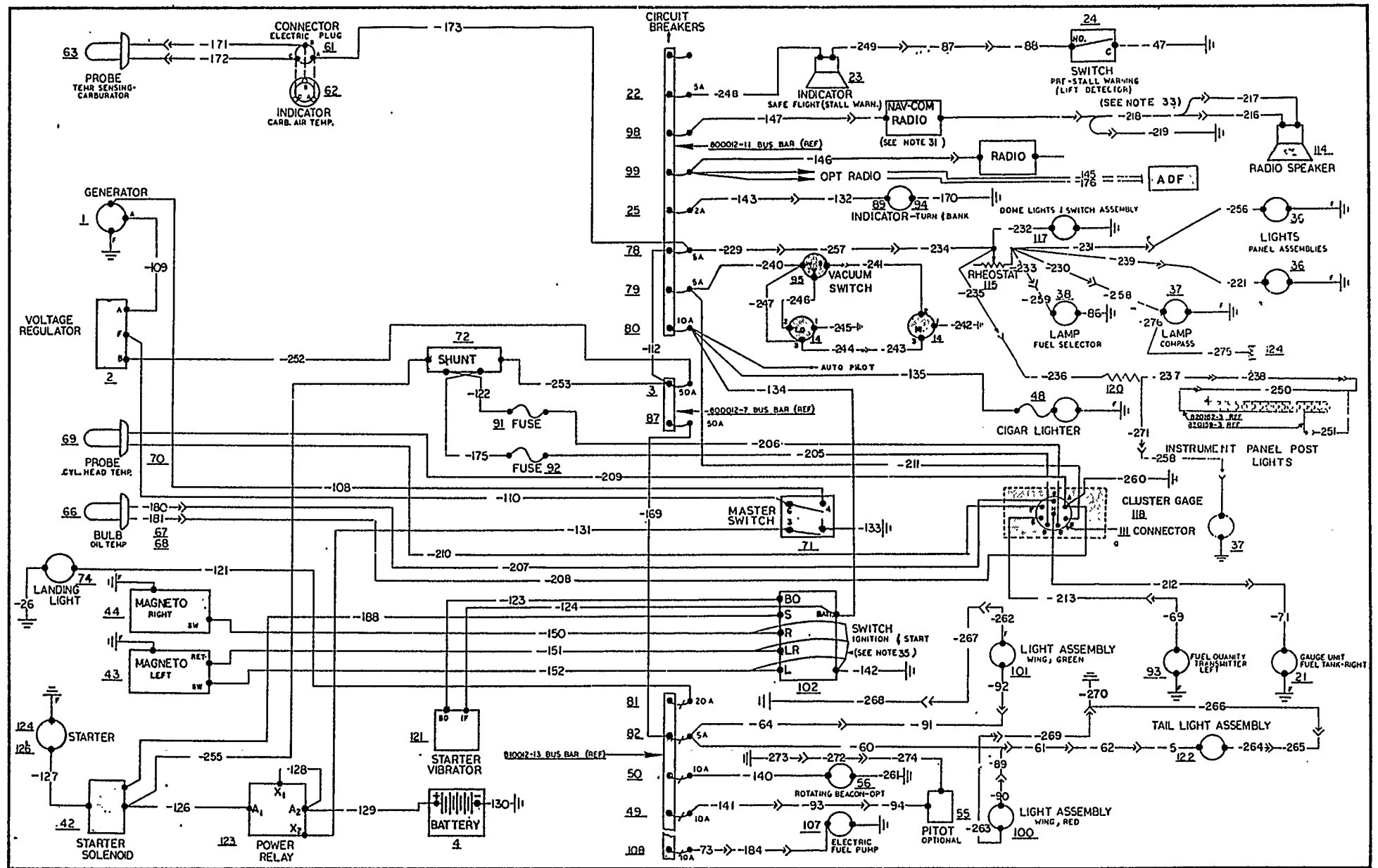
FIGURE 50E. Electrical System (1966 & ON M20D)
