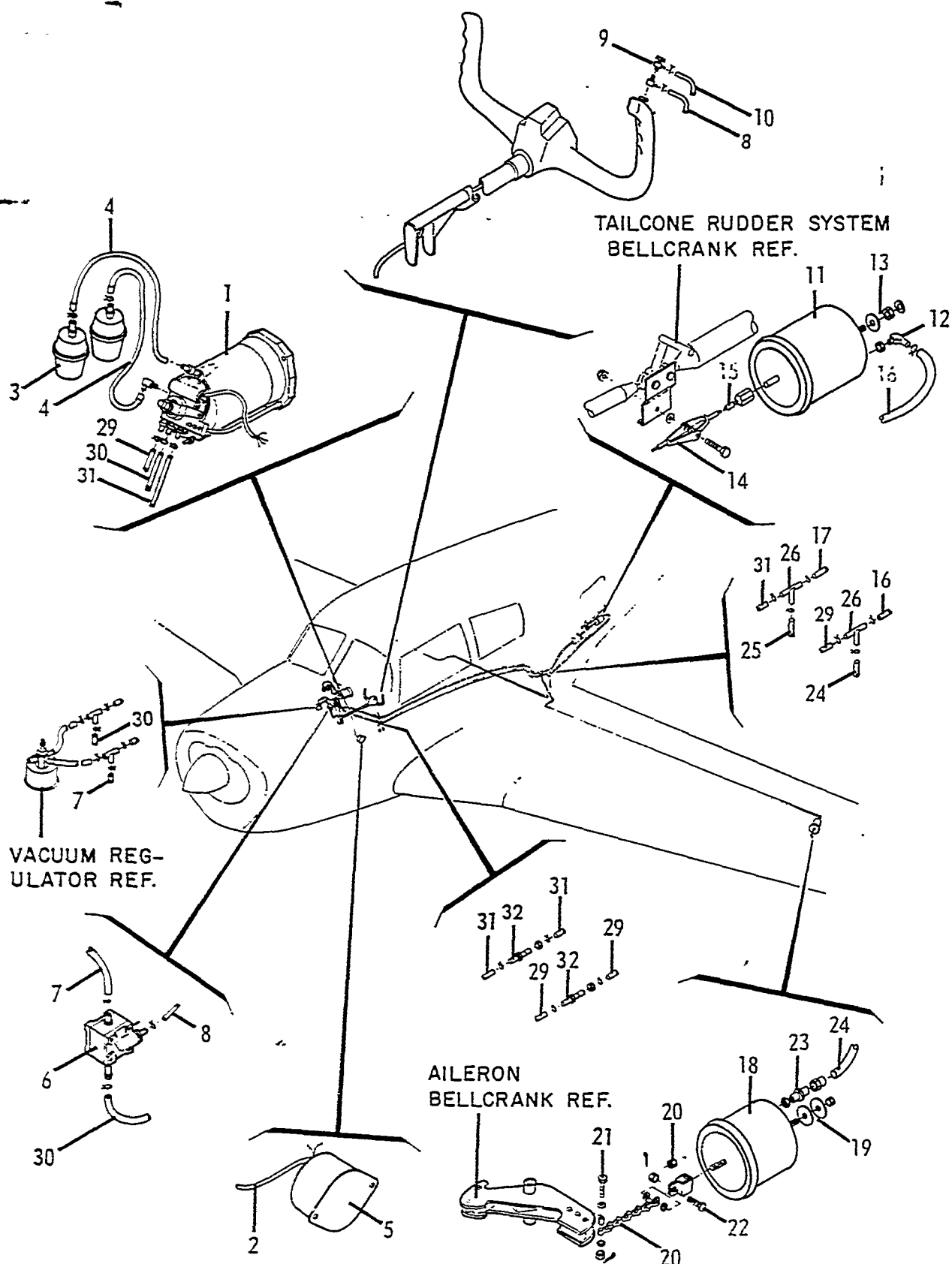
FIGURE 33. Positive Control System (1967 &amp; ON)
