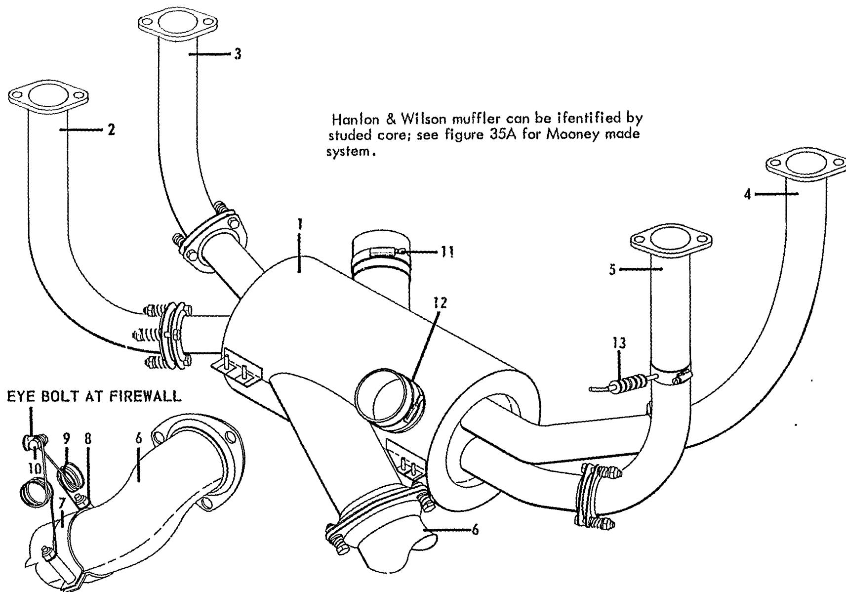
Figure 35, Hanlon & Wilson, Engine Exhaust System
