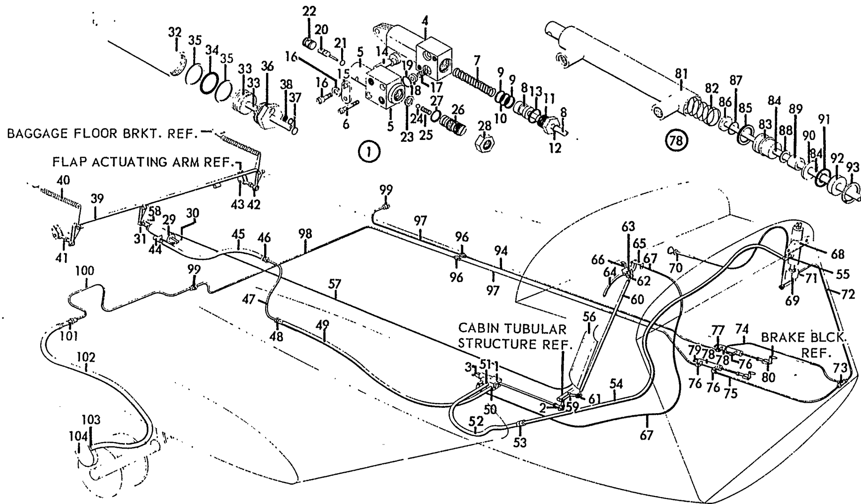
FIGURE 52. Hydraulic Brake & Flap Control Systems
