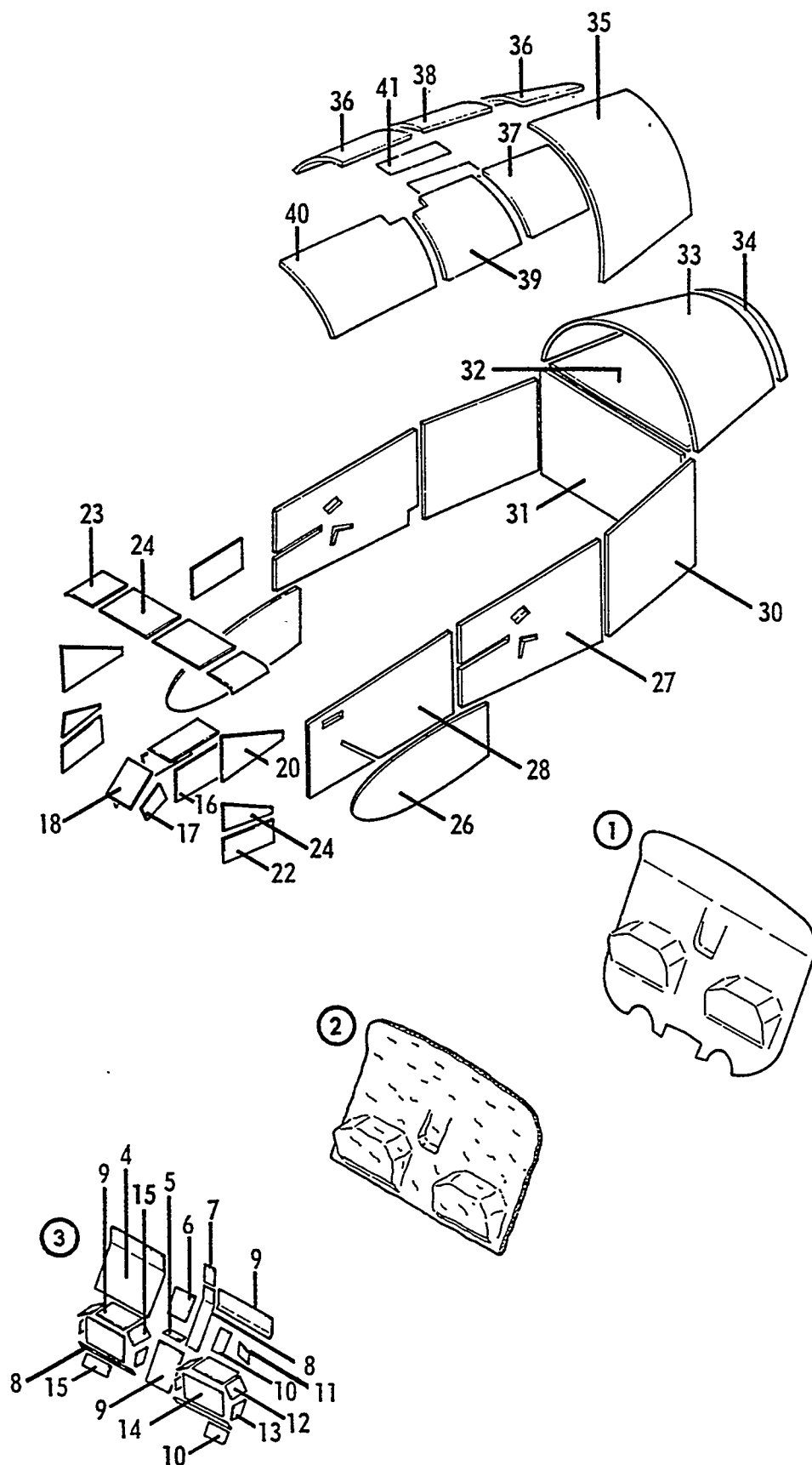
FIGURE 43. Cabin Insulation
