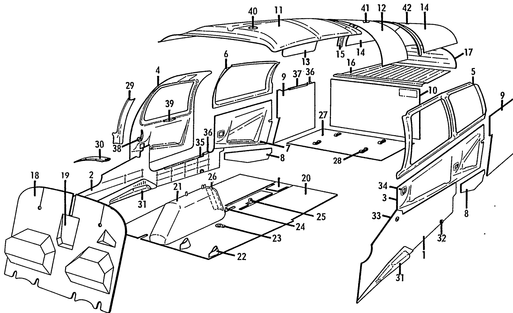
FIGURE 44. Cabin Interior Furnishings (1965 M20C, D&amp;E)
