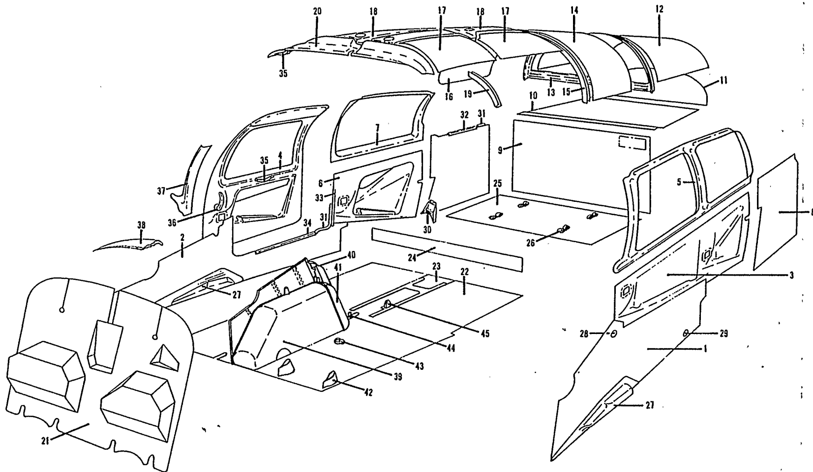
FIGURE 45. Cabin Interior Furnishings (1966 & ON M20C, D&E)
