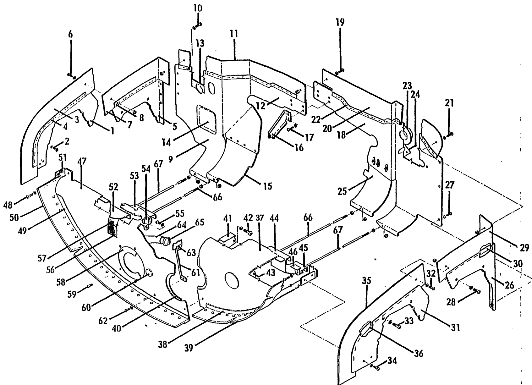
FIGURE 40. Engine Baffle Assembly (1967 &amp; ON)
