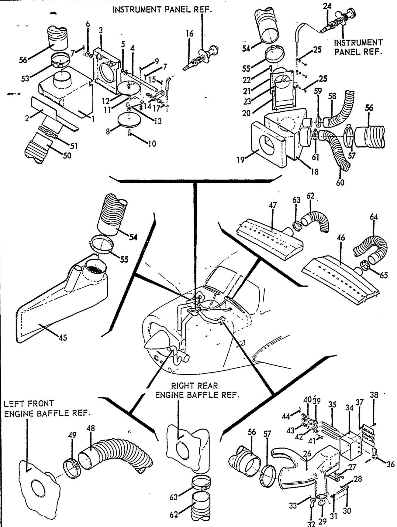
FIGURE 57. Cabin Heating & Cooling System (1967 & ON M20C, E&F)
