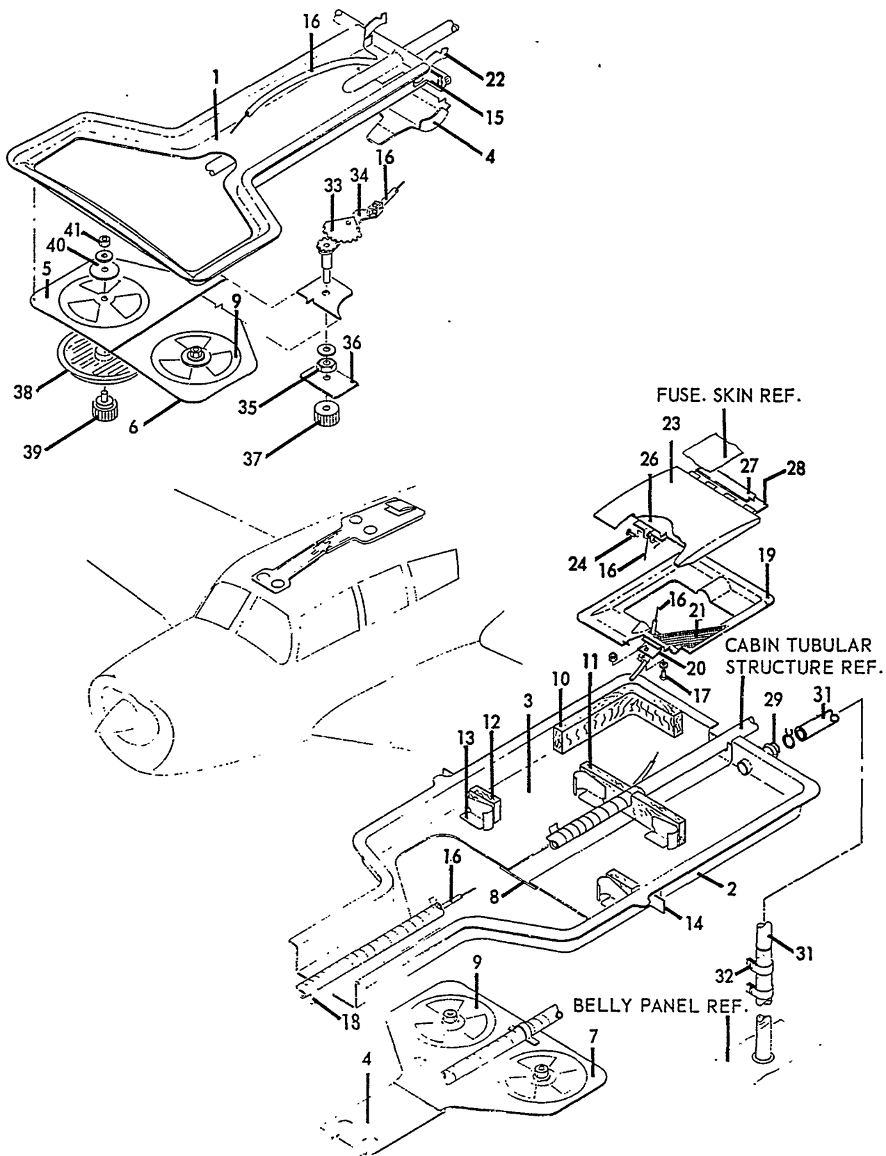
FIGURE 55. Cabin Overhead Ventilation System
