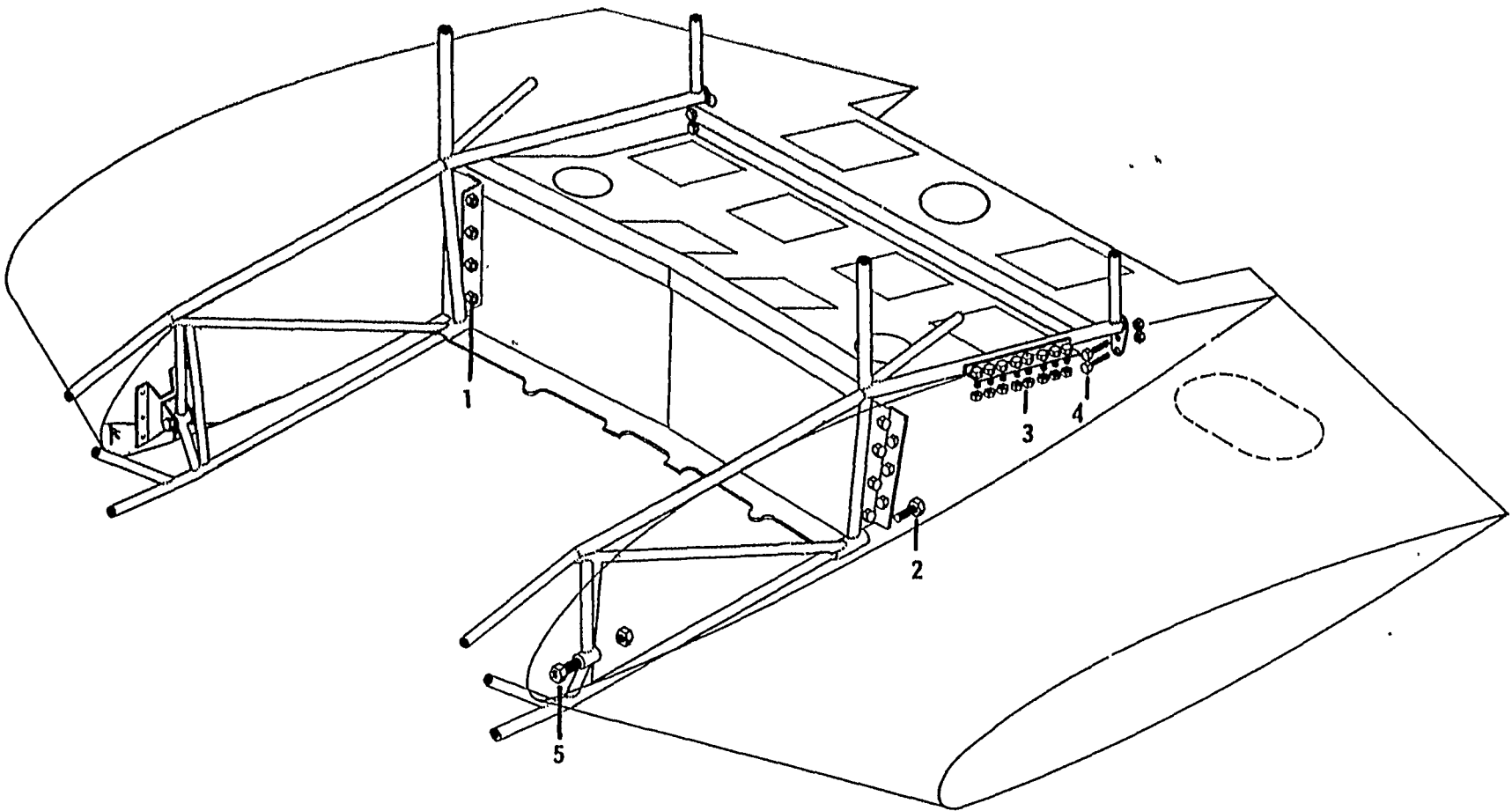
FIGURE 2. Wing Installation
