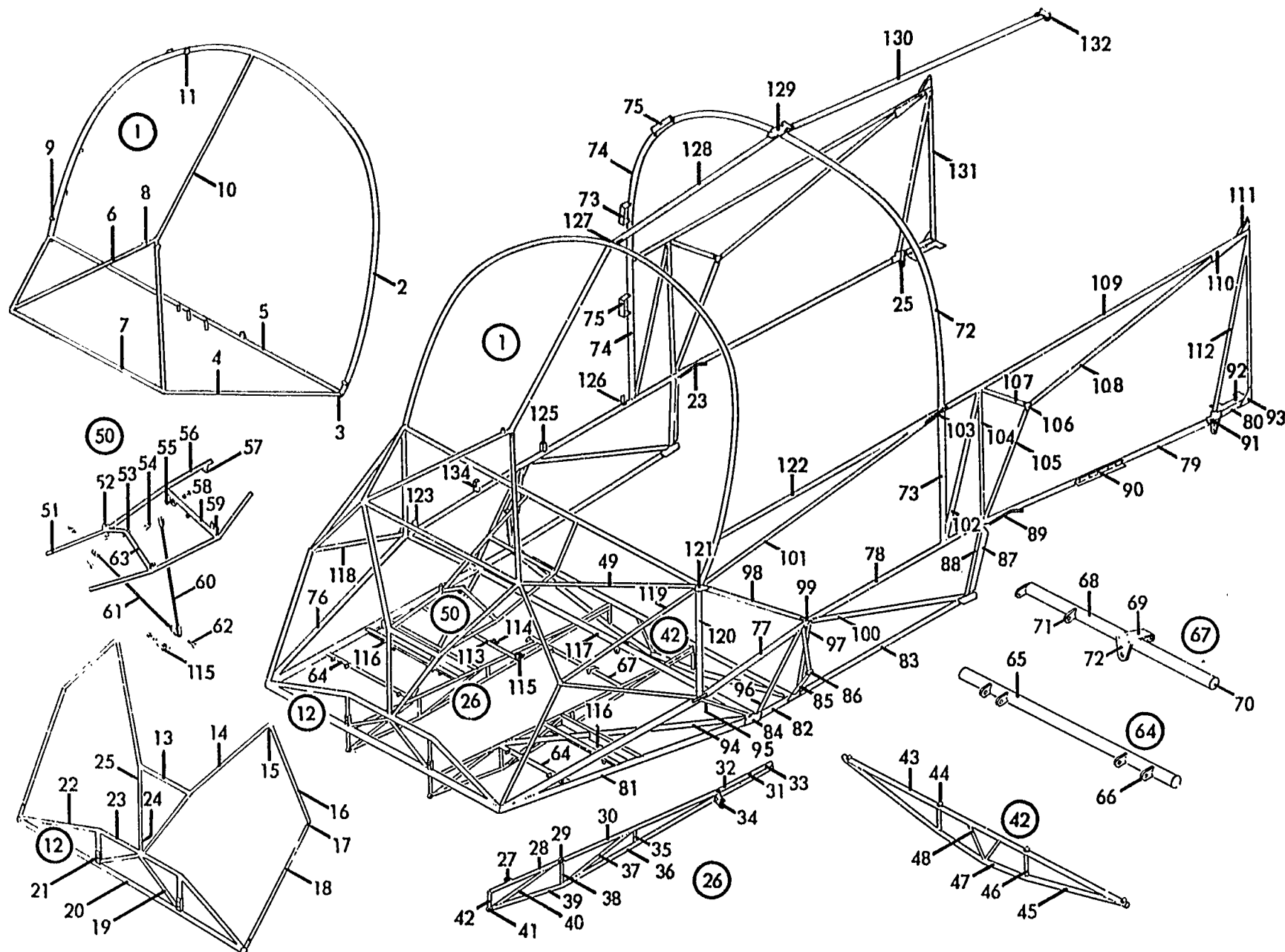
FIGURE 6. Fuselage Tubular Structure Assembly
