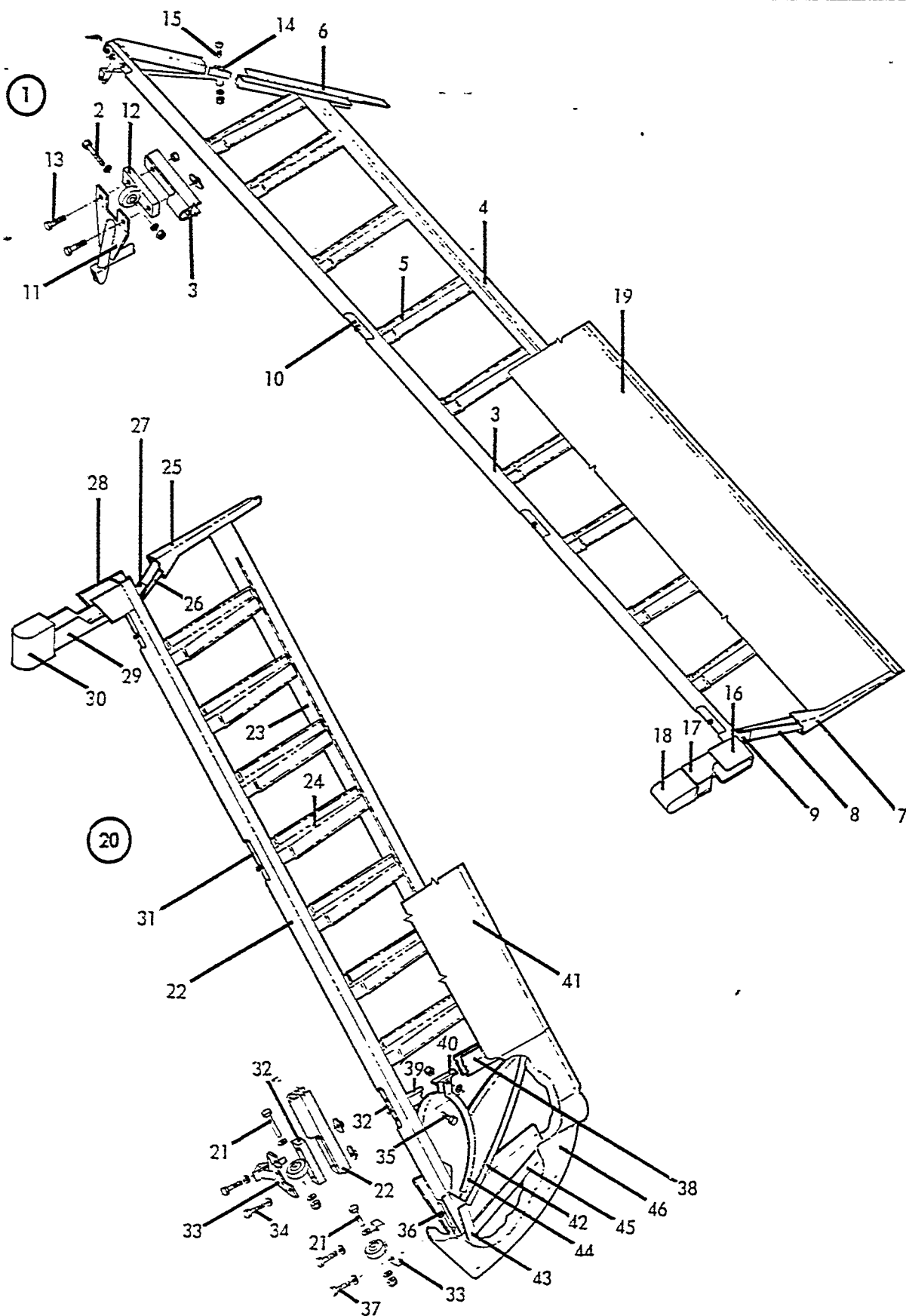
FIGURE 21. Elevator & Rudder Assemblies & Installation
