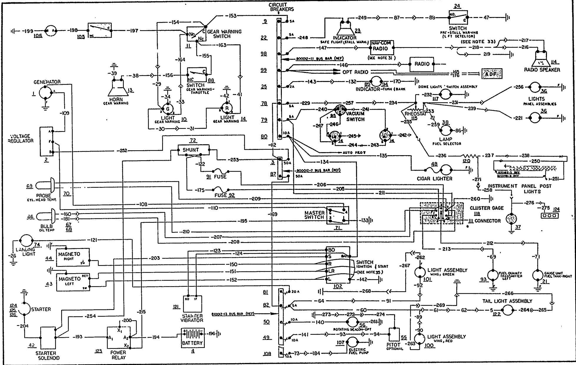
FIGURE 50F. Electrical System (1966 M20E)
