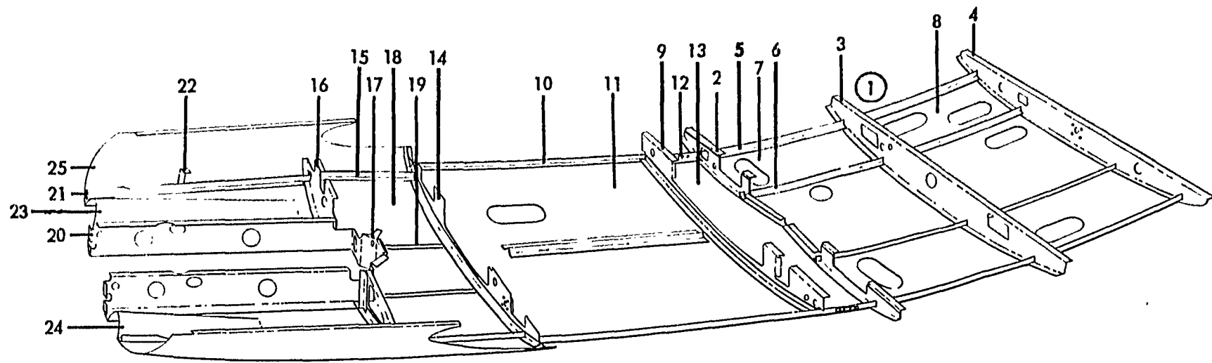
FIGURE 12. Fuselage Bottom Skins & Bulkheads
