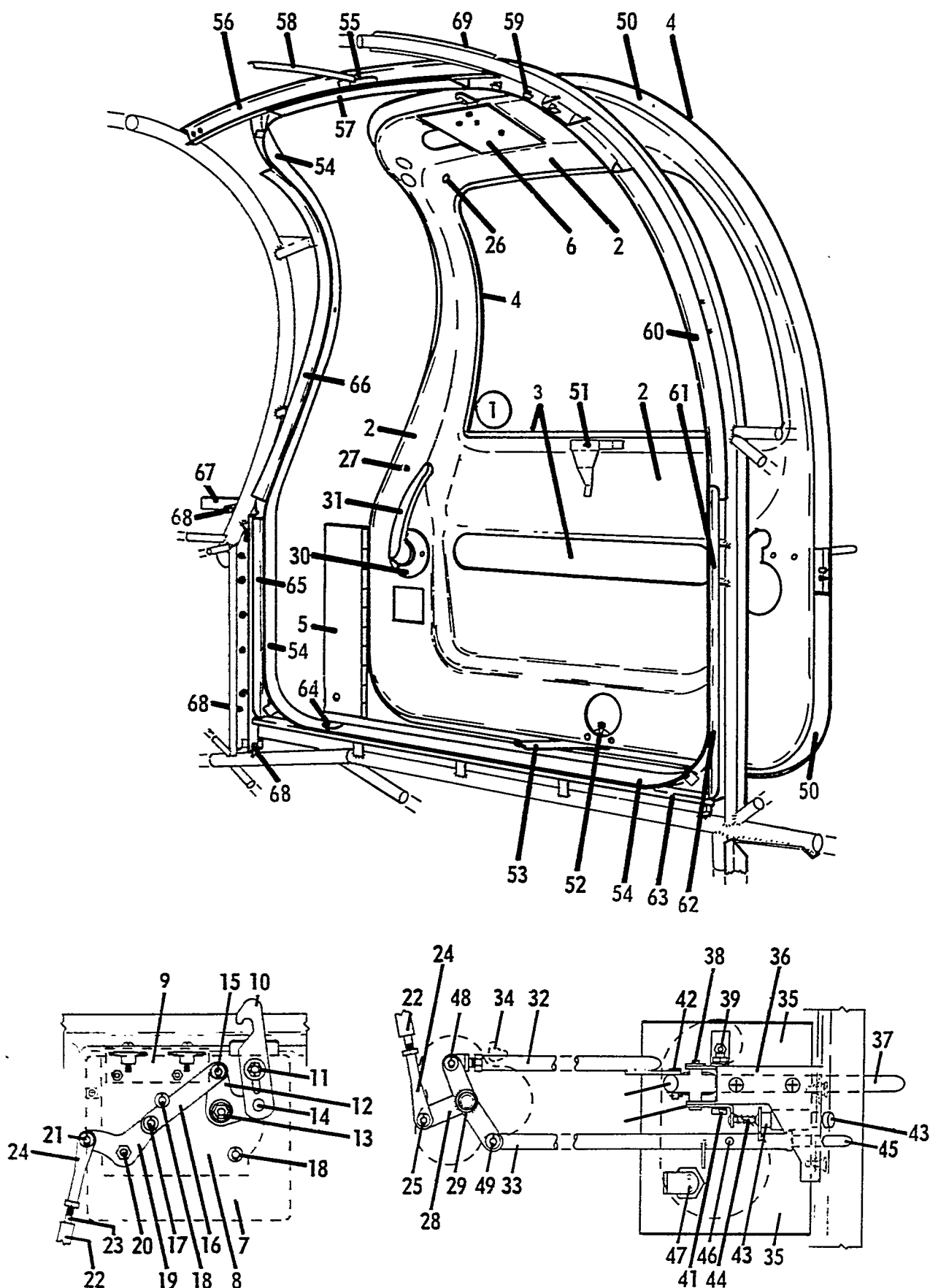
FIGURE 13. Fuselage Cabin Door Assembly
