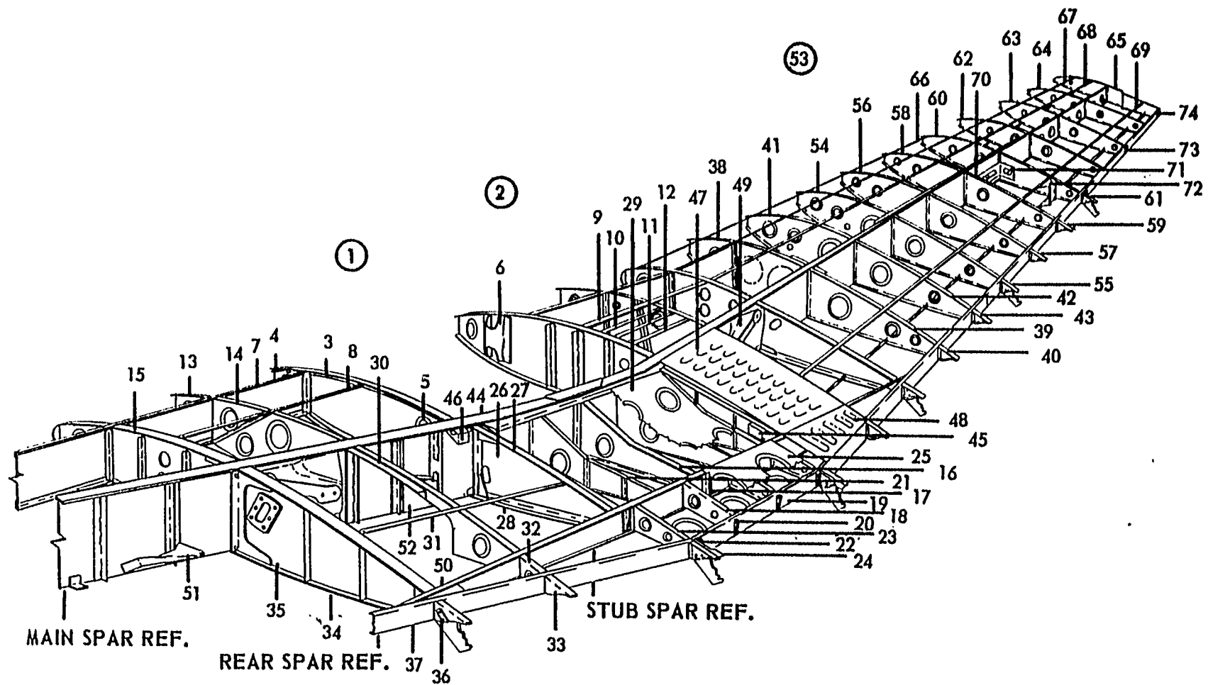
FIGURE 1. Wing Assembly
