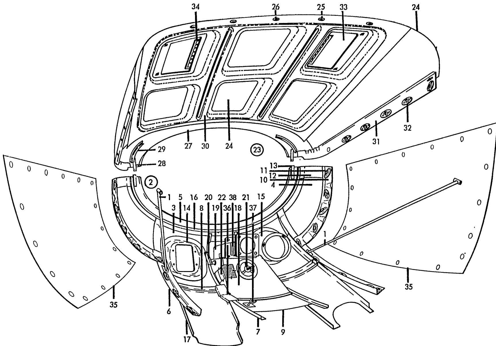
FIGURE 42. Engine Cowling Assembly (1966 & ON)
