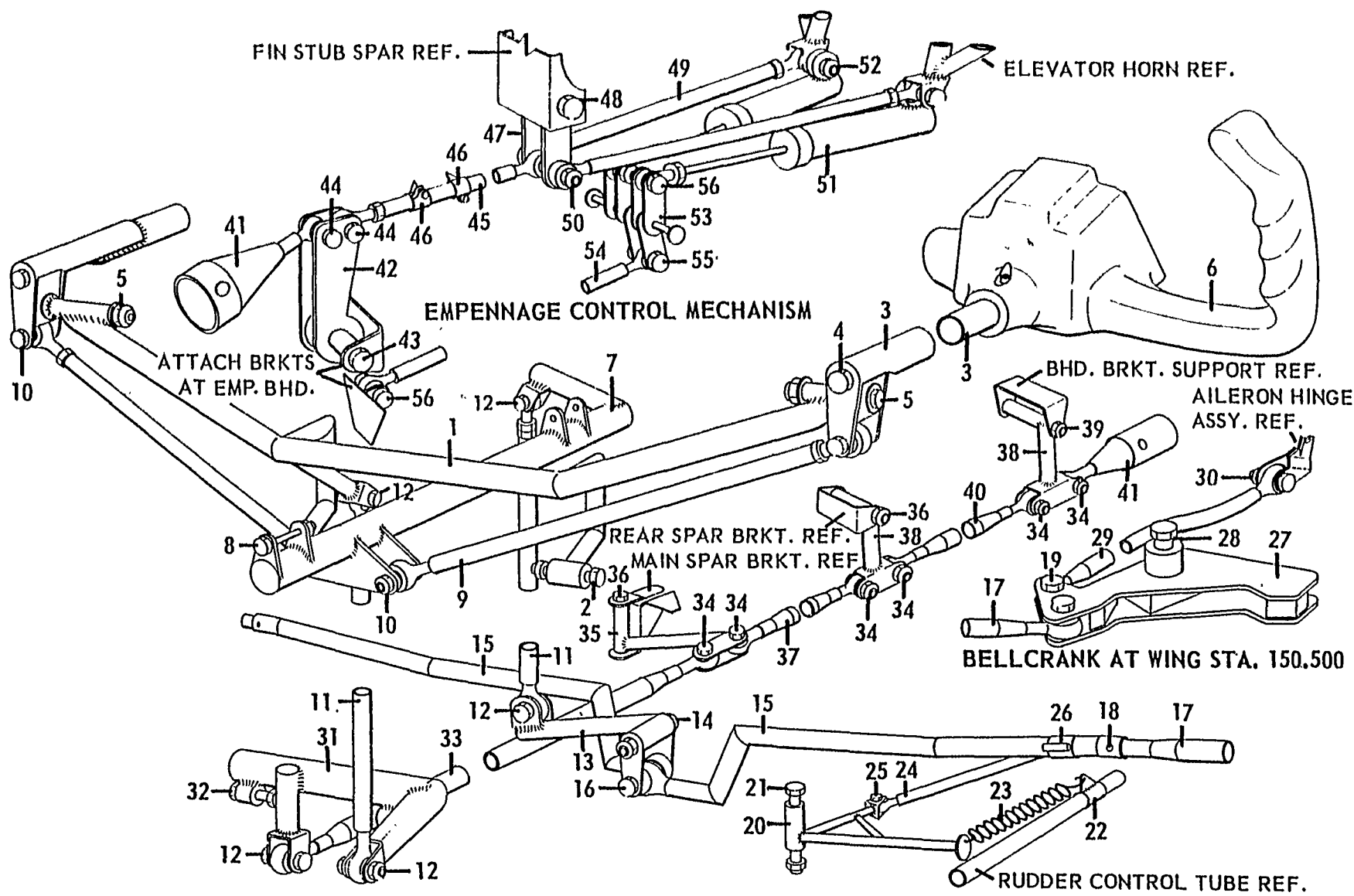
FIGURE 28. Elevator & Aileron Control Systems
