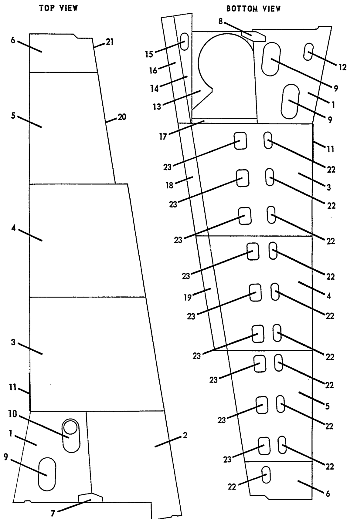
FIGURE 4. Wing Skins & Inspection Covers
