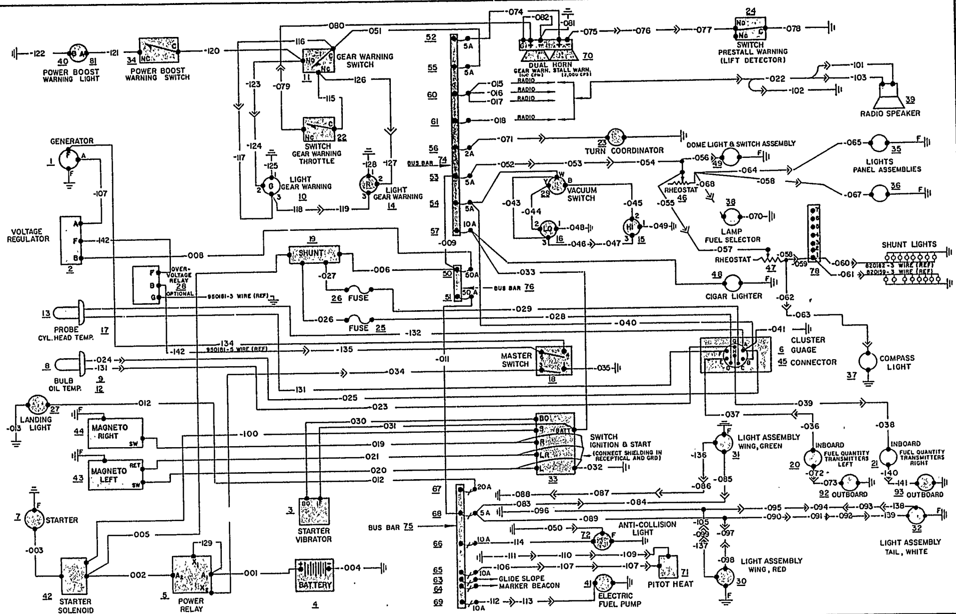
FIGURE 51. Electrical System (1967 & ON M20F)
